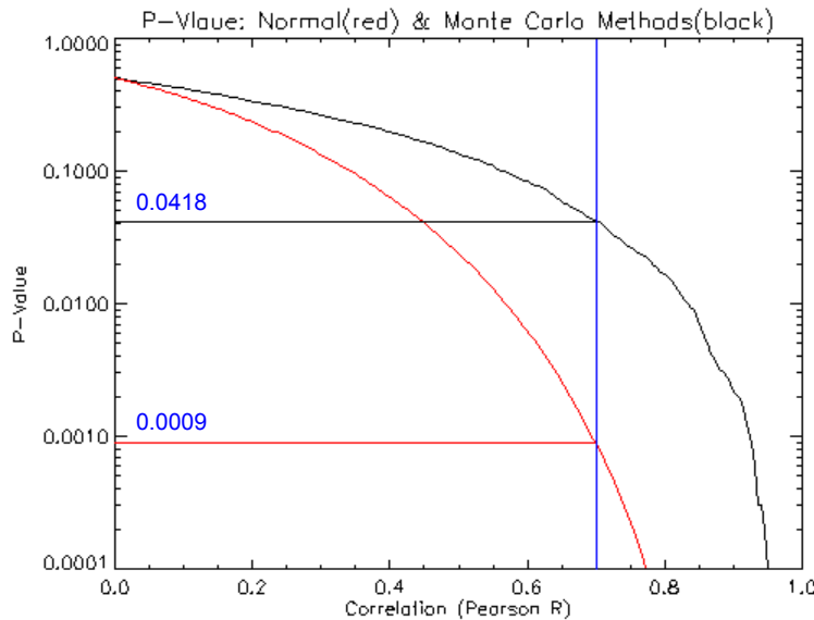
Figure 7. P-Values Under a Normal and Monte Carlo Assumption.
