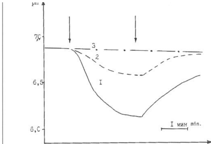
Figure 2. Typical changes of pH during the operator's effect (the arrows show the beginning and end of the operator's effort period): 1-distilled water; 2-salt solution; 3-non-stirred solution.
