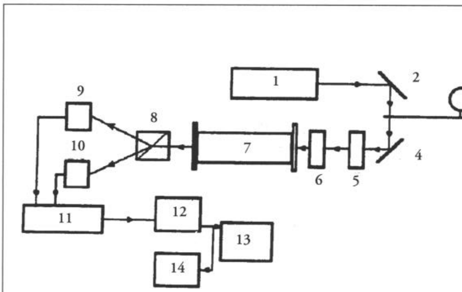
Figure 1. A diagram of the system for measuring optical activity of liquid media: (1) He- laser (wavelength 0.63 micrometers); (2,4) reflecting mirrors; (3) shutter; (5,6) polarizers; (7) cuvette with solution; (8) Glan-Thompson prism; (9,10) photodetectors; (11) comparison block; (12) amplifier; (13) oscilloscope; (14) strip-chart recorder.
